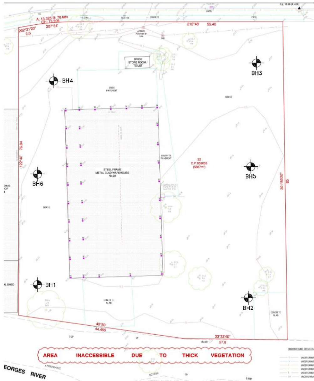
Figure 8: Borehole locations (Source: Asset Geotechnical)
